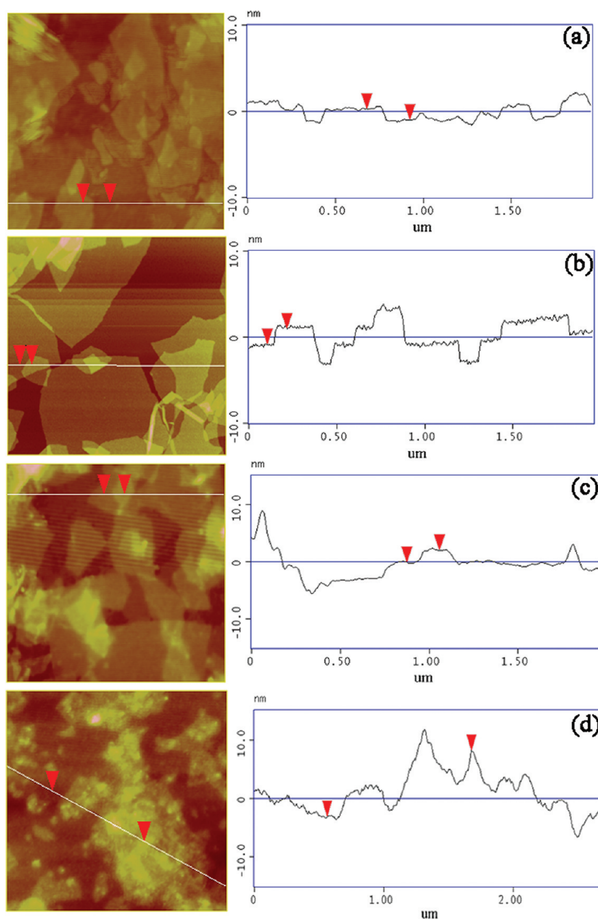
Figure 3. AFM images and height profiles of (a) GO, (b) CD-G, and HGIC (c) at room temperature and (d) at 40 °C above the LCST.
